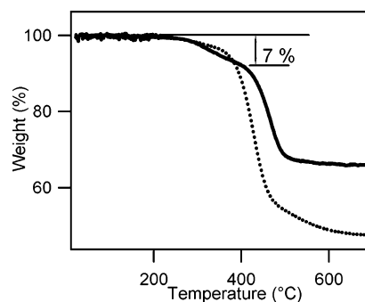
Figure 5. TGA analyses of 1,4-TPPE (dotted line) and 1,4-addMe (solid line) under \text{N}_2 ( 10 \text{ }^\circ\text{C}\cdot\text{min}^{-1} heating rate).
